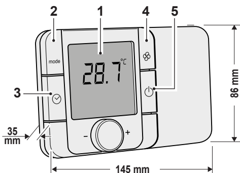
B0860 (wall version) Compatible with wall box type 803
